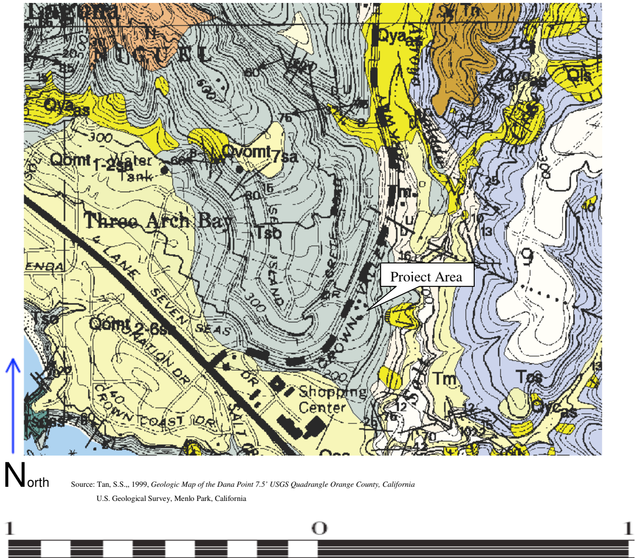
Figure 2 – Regional Geology
