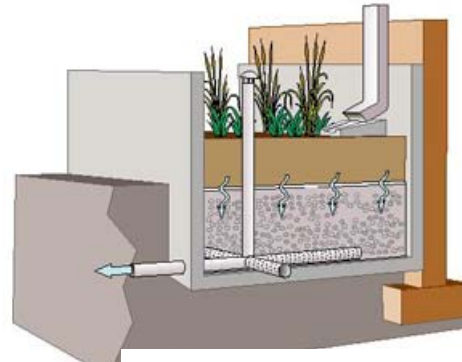
Flow-through Planter
