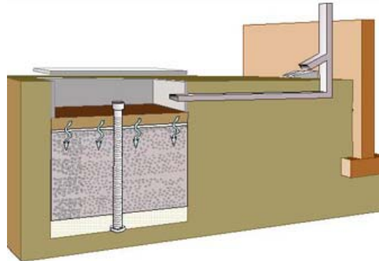
Dry Well
